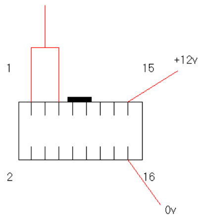
CCTalk Bus
